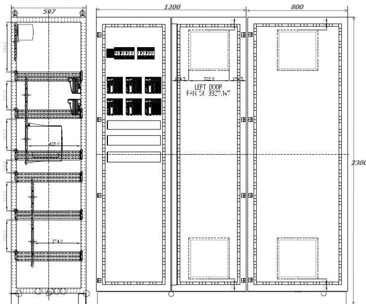
Stand Alone Cabine dimentionis
